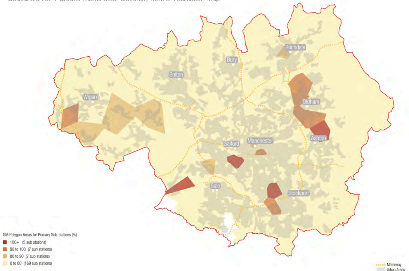
^ Spatial plan 5.2: Greater Manchester electricity network fault level thresholds
