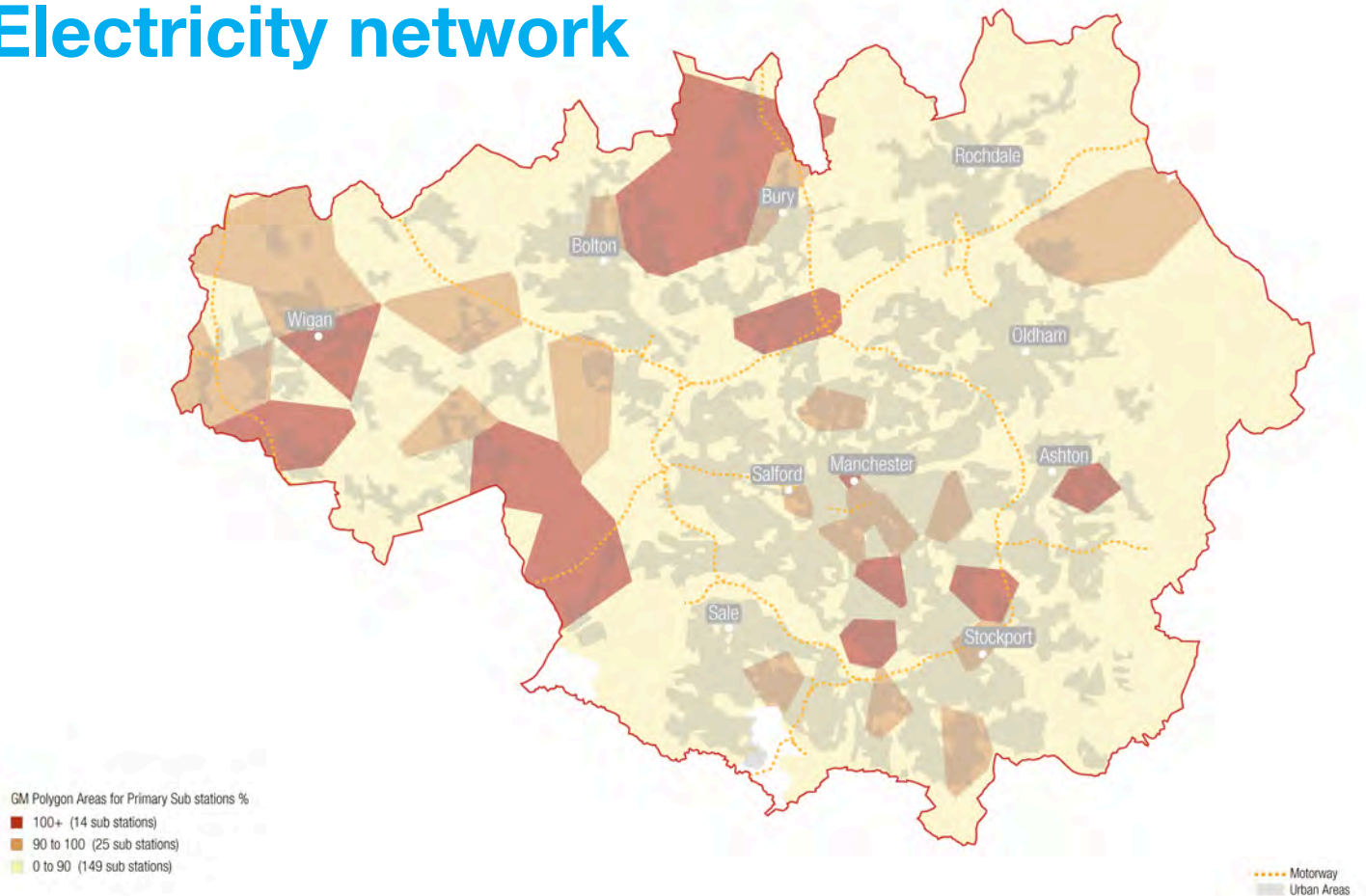
^ Spatial plan 5.1: Greater Manchester electricity network utilisation map
