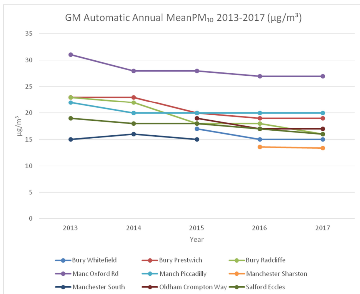
Figure 3.4- Trends in Annual Mean PM 10 Concentrations Measured at Automatic Monitoring Sites – Bury - Salford
