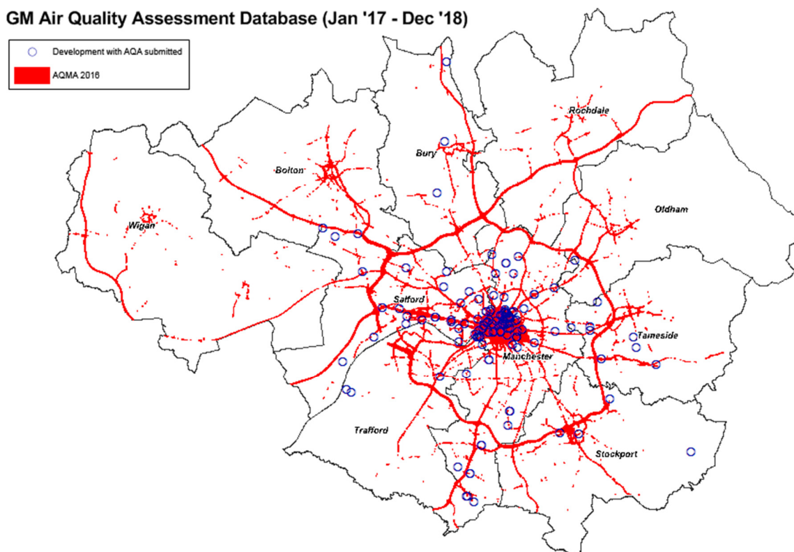
Figure 2.1 Maps showing Air Quality Assessment cumulative database.
