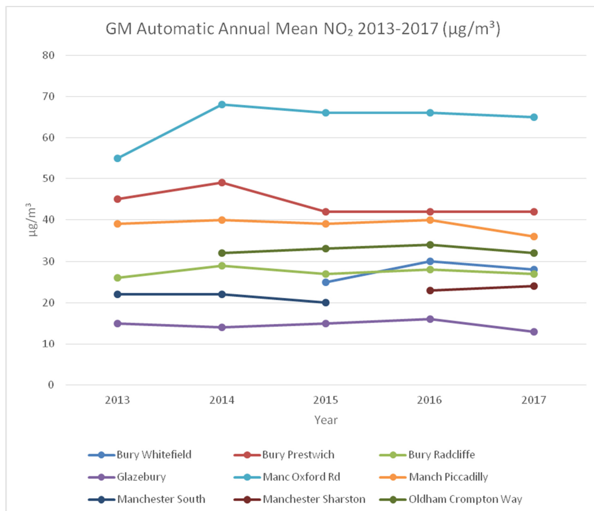
Figure 3.1 - Trends in Annual Mean NO 2 Concentrations Measured at Automatic Monitoring Sites Bury – Oldham.
