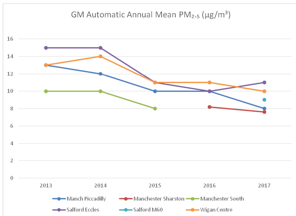
Figure 3.6 - Trends in Annual Mean PM 2.5 Concentrations Measured at Automatic Monitoring Sites
